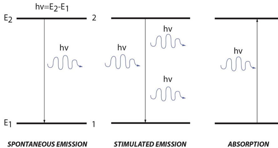
Figure 2: Primary mechanisms for energy transfer [4]
